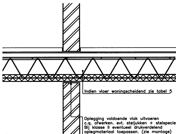
Detail III
