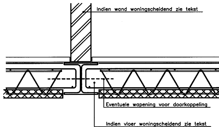
Detail Xb
