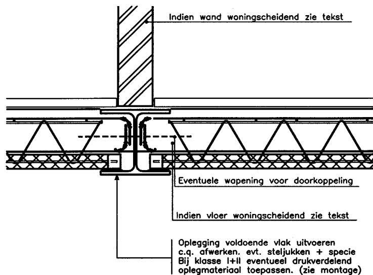
Detail Xd
