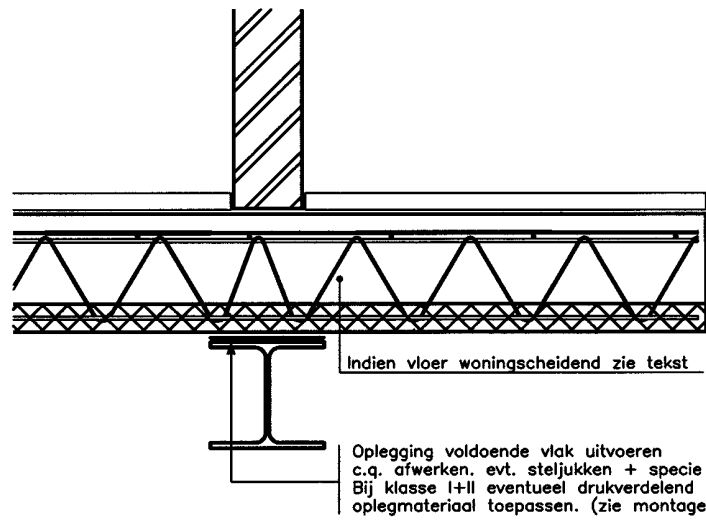
Detail Xb
