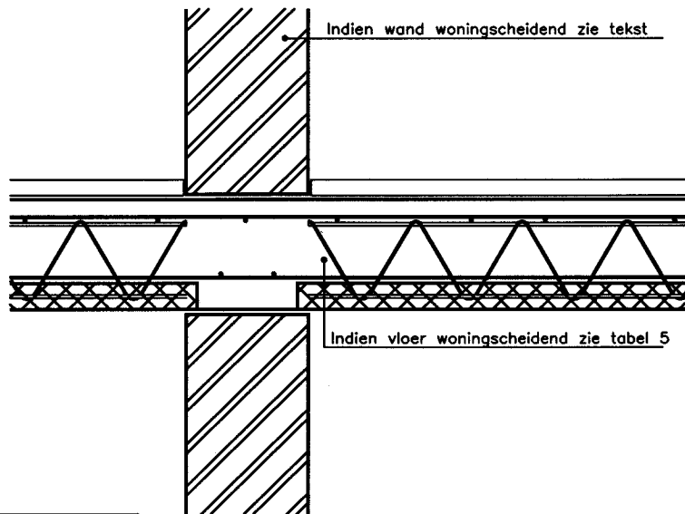
Detail II
