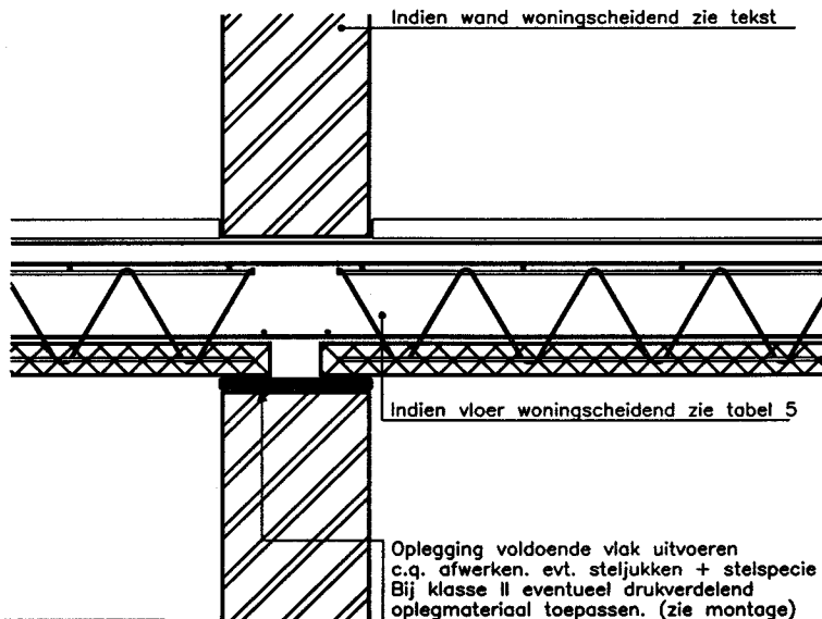
Detail IIa
