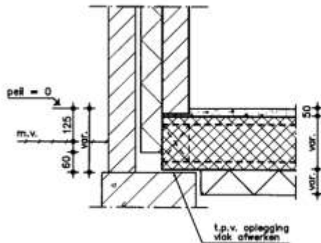
begingrond detail 21
