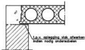
verdieping detail 16
