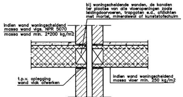
beganegrond detail 20
