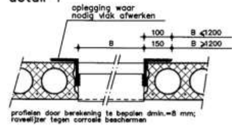
detail 4
