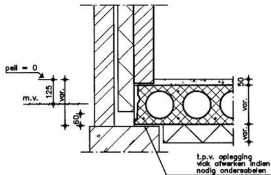
beganegrond detail 19
