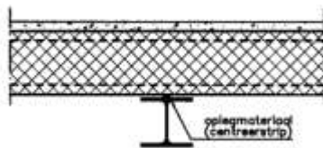
verdieping detail 11
