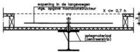
detail 12 – sleufsparing
