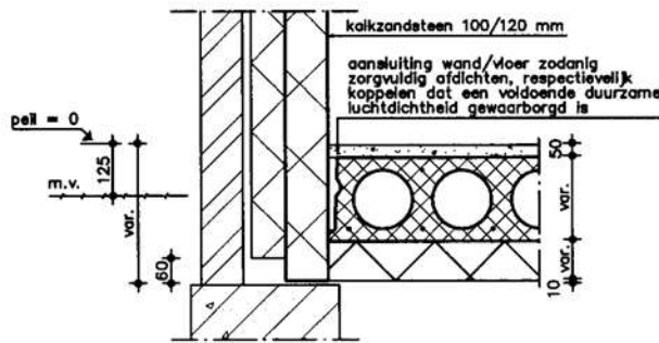
beganegrond kalkzandstendetail 10
