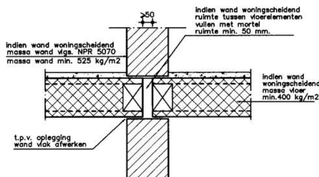
verdieping detail 5
