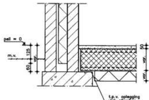
begingrond detail 22
