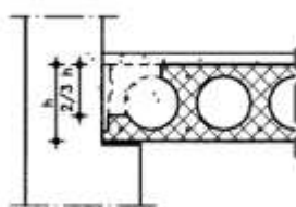
verdieping detail 15
