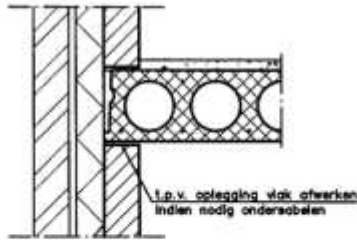
verdieping detail 9
